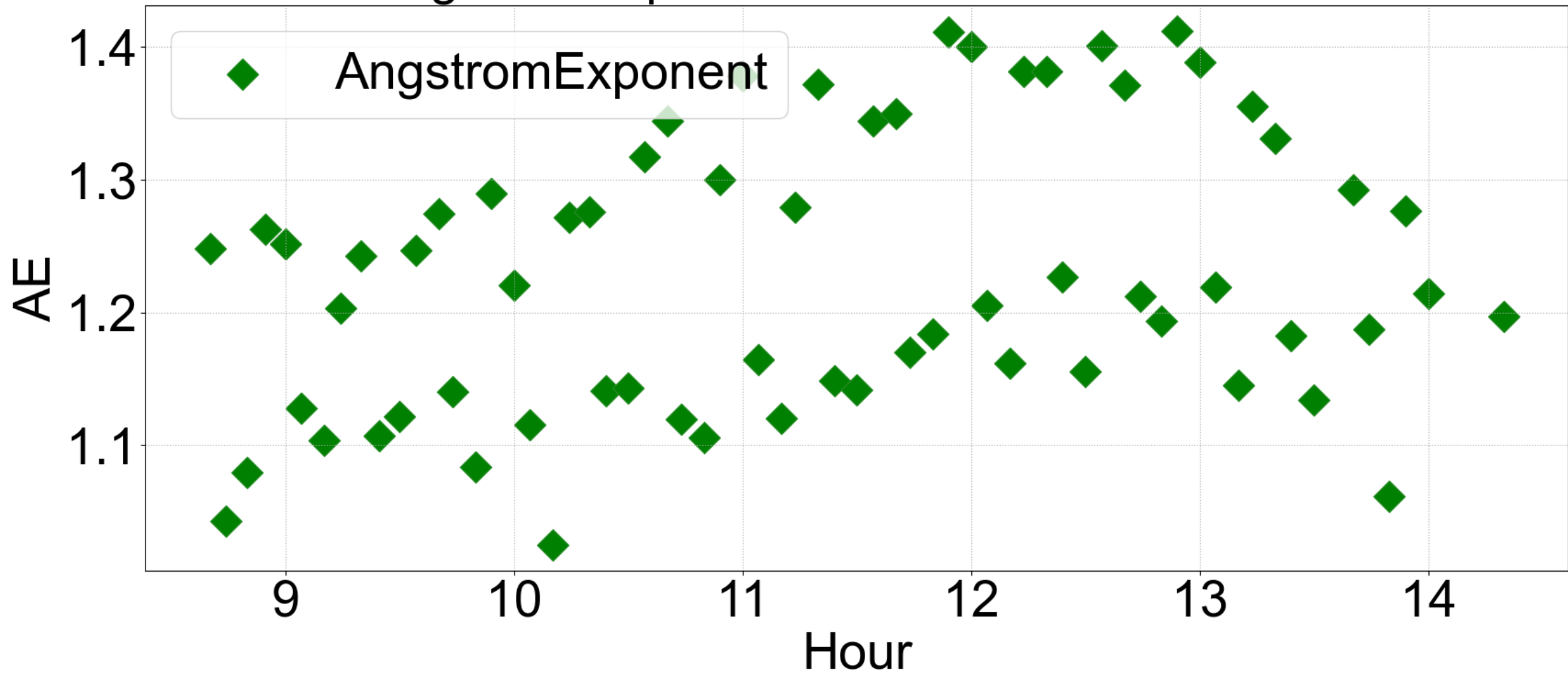
AngstromExponent in Chiba for 2023.12.04
