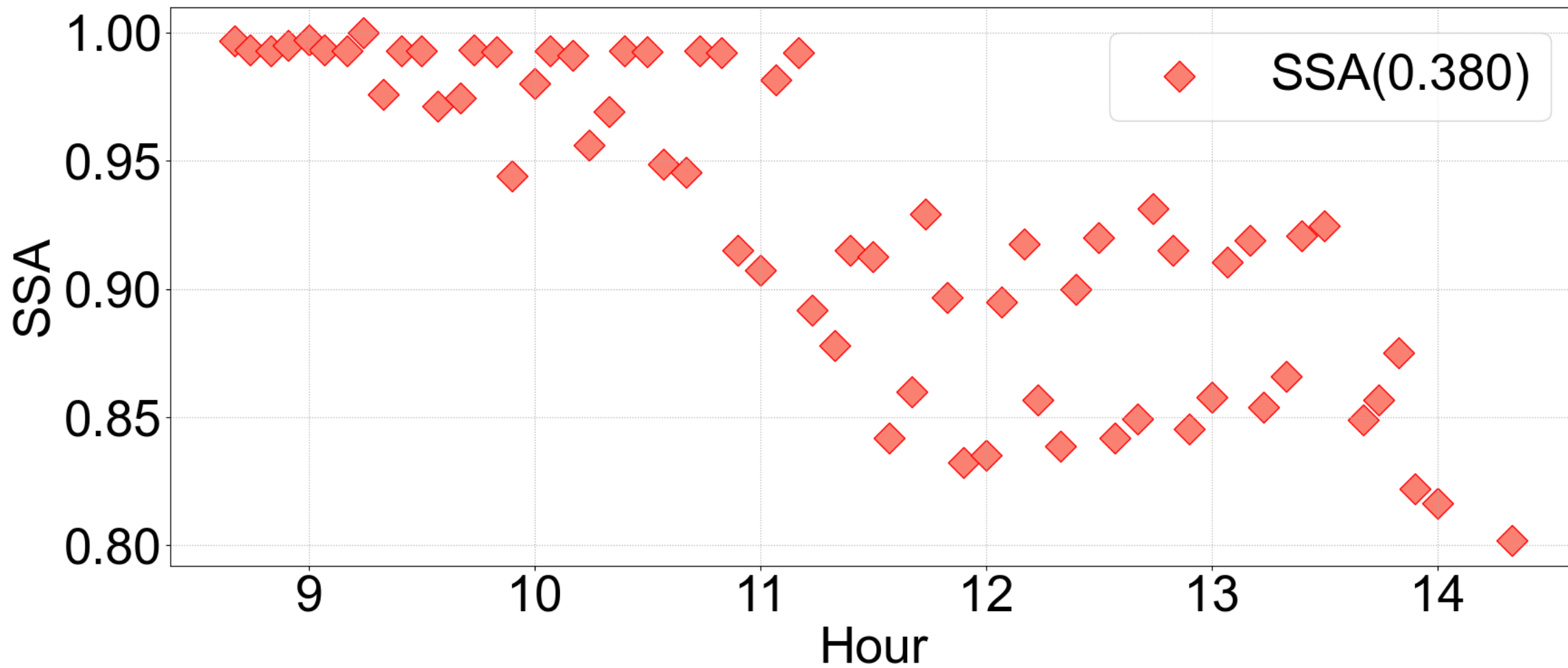
SSA in Chiba for 2023.12.04
