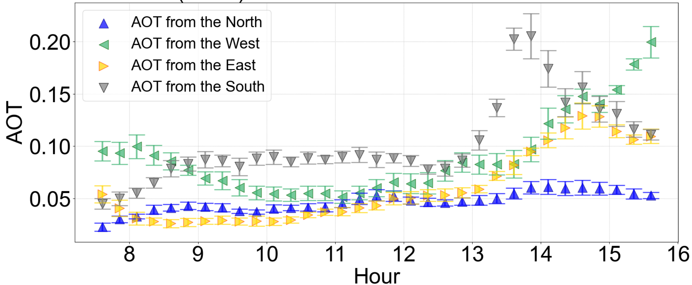
AOT(0.357) of MAX-DOAS in Chiba for 2023.12.04
